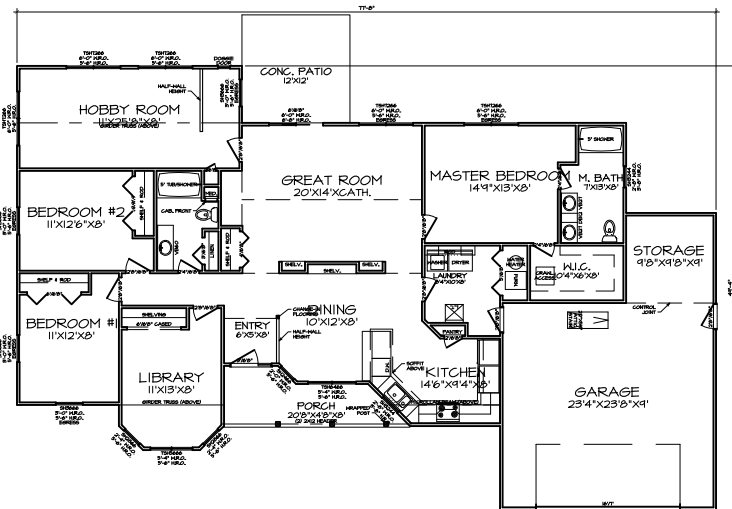
1 FIRST FLOOR PLAN A-3
