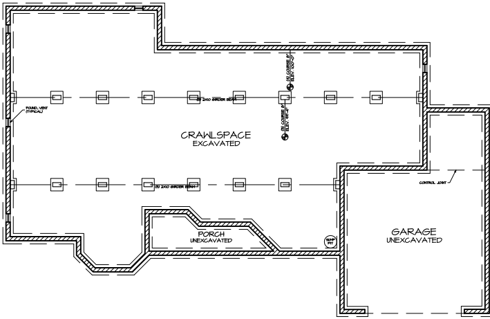
1 FOUNDATION PLAN A-2
